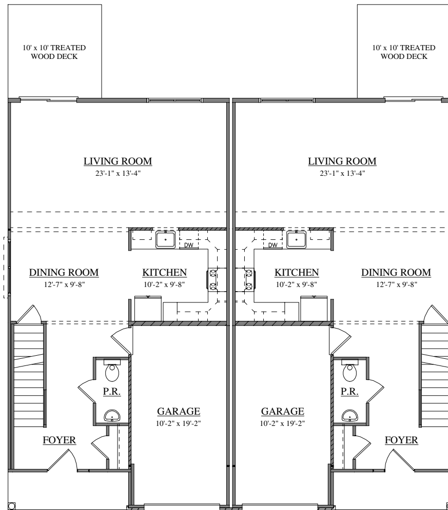
FIRST FLOOR PLAN FORINO - BERKELEY TOWNHOUSE
