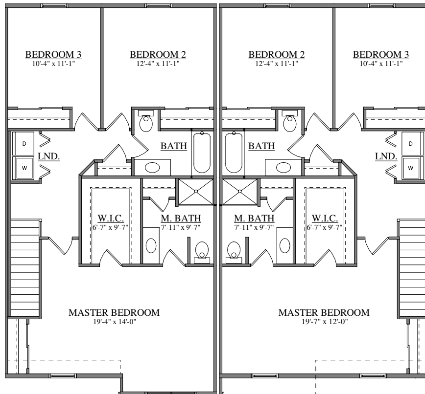
SECOND FLOOR PLAN FORINO - BERKELEY TOWNHOUSE
