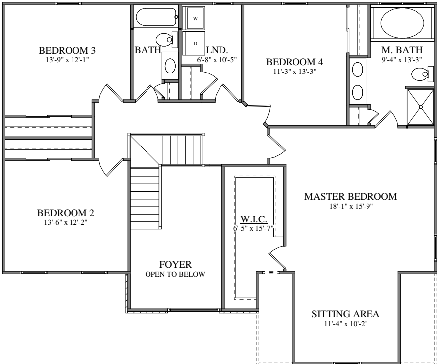
SECOND FLOOR PLAN FORINO - BOSTON
