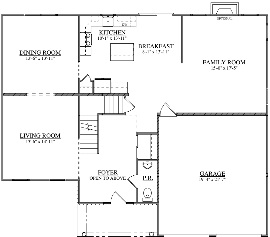
FIRST FLOOR PLAN FORINO - BOSTON
