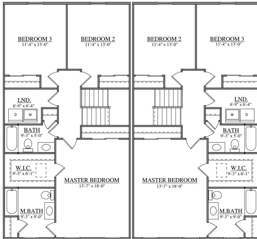
SECOND FLOOR PLAN FORINO - CARNEGIE TOWNHOUSE
