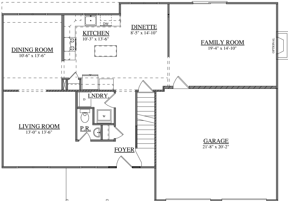
FIRST FLOOR PLAN FORINO - DENVER I - 4BR
