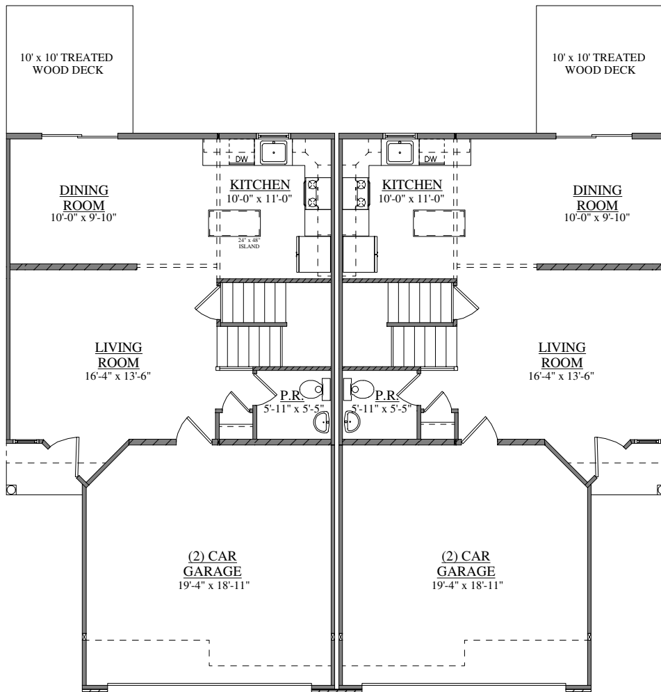
FIRST FLOOR PLAN FORINO - DURHAM TOWNHOUSE
