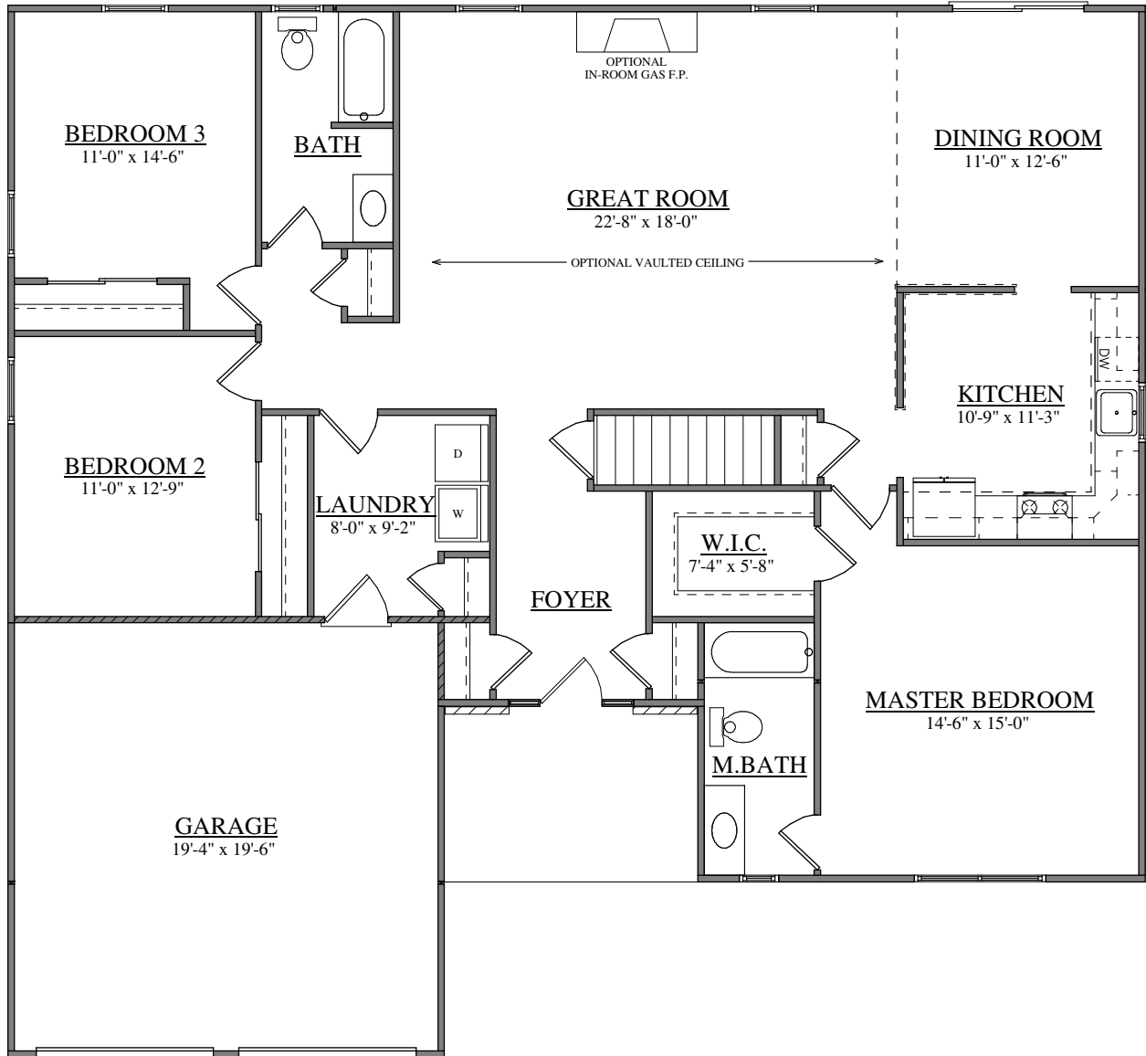
FIRST FLOOR PLAN FORINO - FLORIDA
