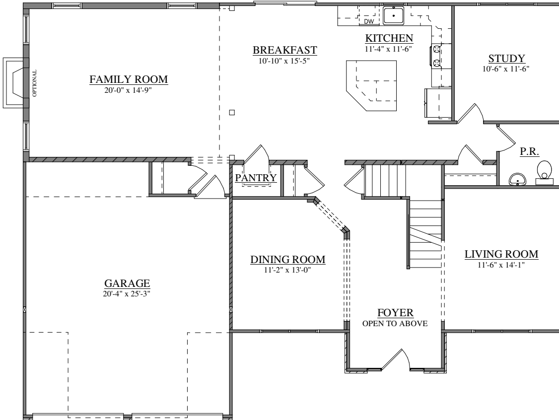
FIRST FLOOR PLAN FORINO - KENNEDY I
