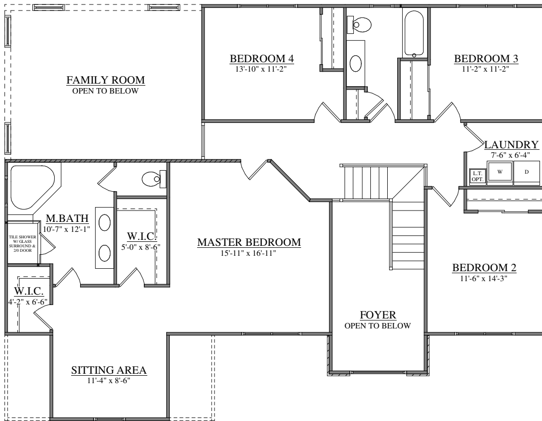
SECOND FLOOR PLAN FORINO - KENNEDY I
