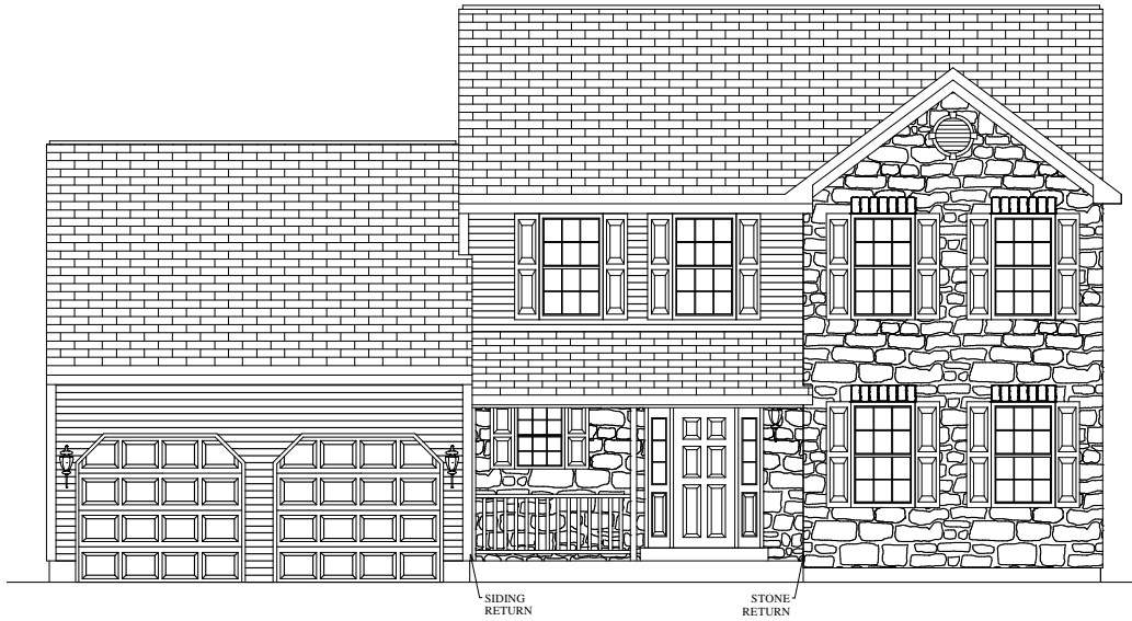
FRONT ELEVATION FORINO - NEBRASKA II - STANDARD CLASSIC 2303 SQ. FT.
