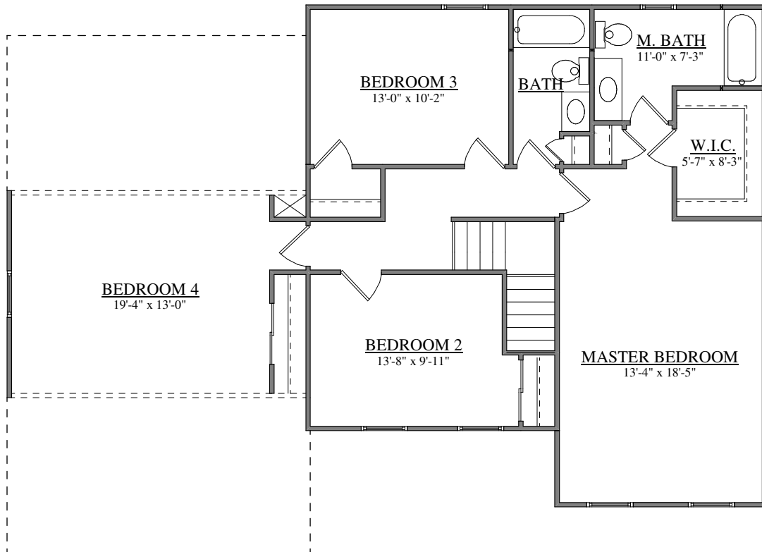
SECOND FLOOR PLAN FORINO - NEBRASKA
