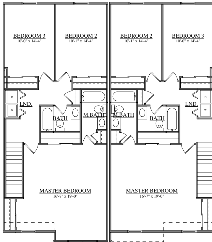
SECOND FLOOR PLAN FORINO - OXFORD TOWNHOUSE
