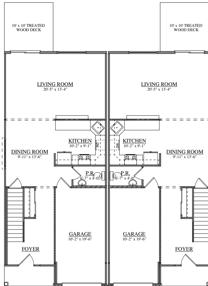
FIRST FLOOR PLAN FORINO - OXFORD TOWNHOUSE
