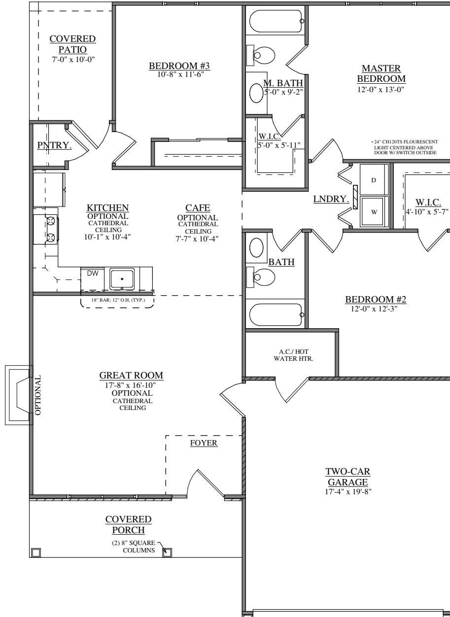
FIRST FLOOR PLAN FORINO - VIRGINIA
