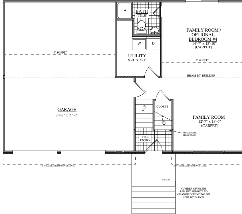
LOWER LEVEL PLAN FORINO - THE COOSAW (S.C.#9)
