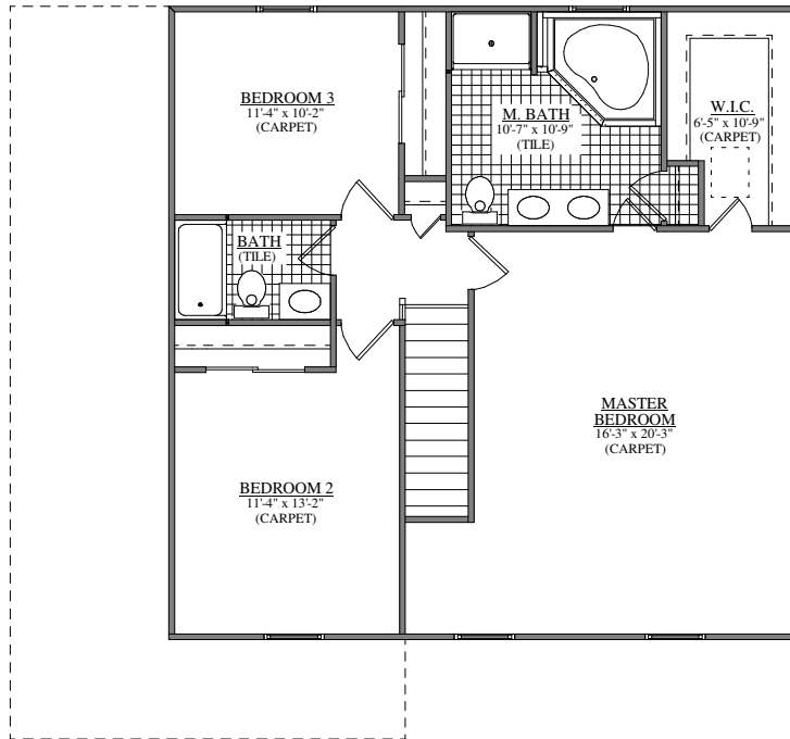
SECOND FLOOR PLAN FORINO - THE SALUDA (S.C. #5)
