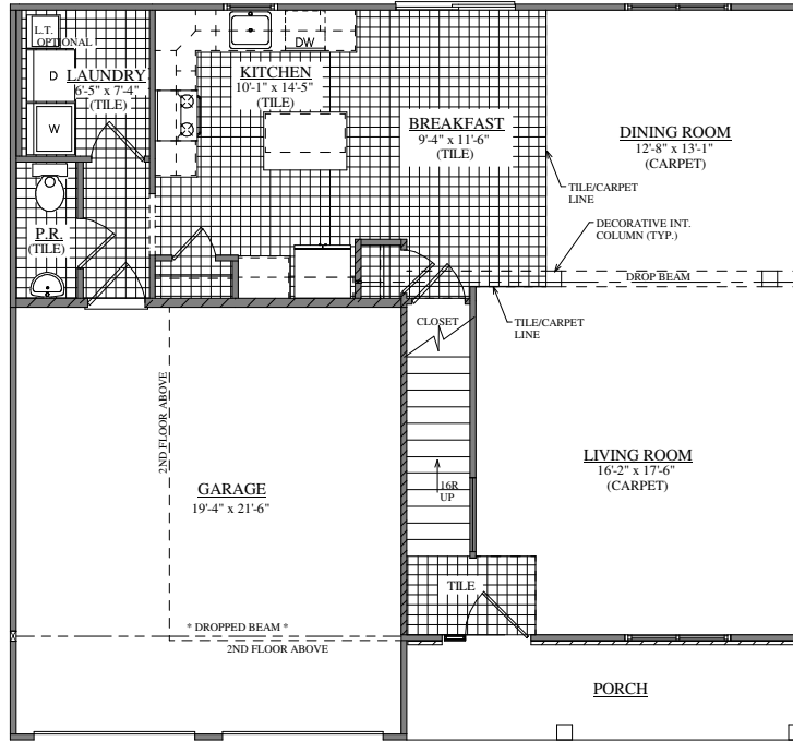
FIRST FLOOR PLAN FORINO - THE SALUDA (S.C. #5)
