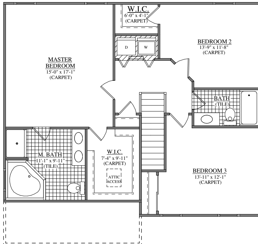
SECOND FLOOR PLAN FORINO - THE BEAUFORT (S.C. #15)
