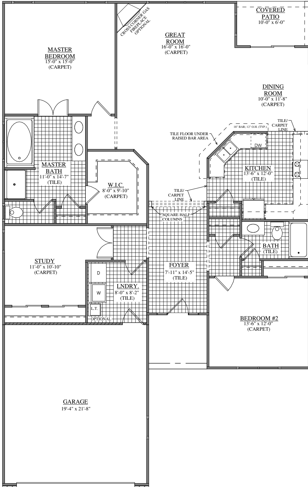
FIRST FLOOR PLAN FORINO - THE ASHLEY (S.C. #1)
