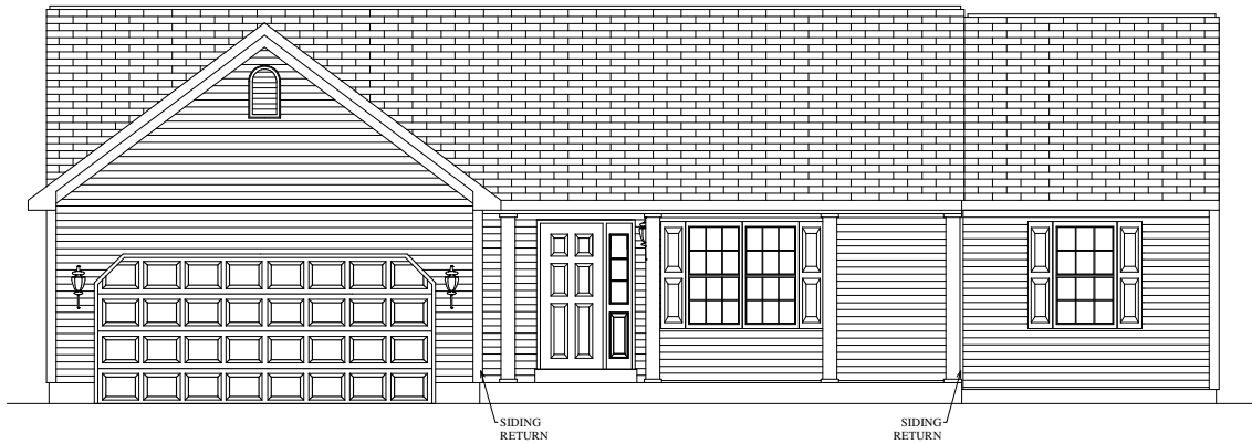
FRONT ELEVATION FORINO - AUSTIN I - STANDARD CLASSIC 1355 SQ. FT.
