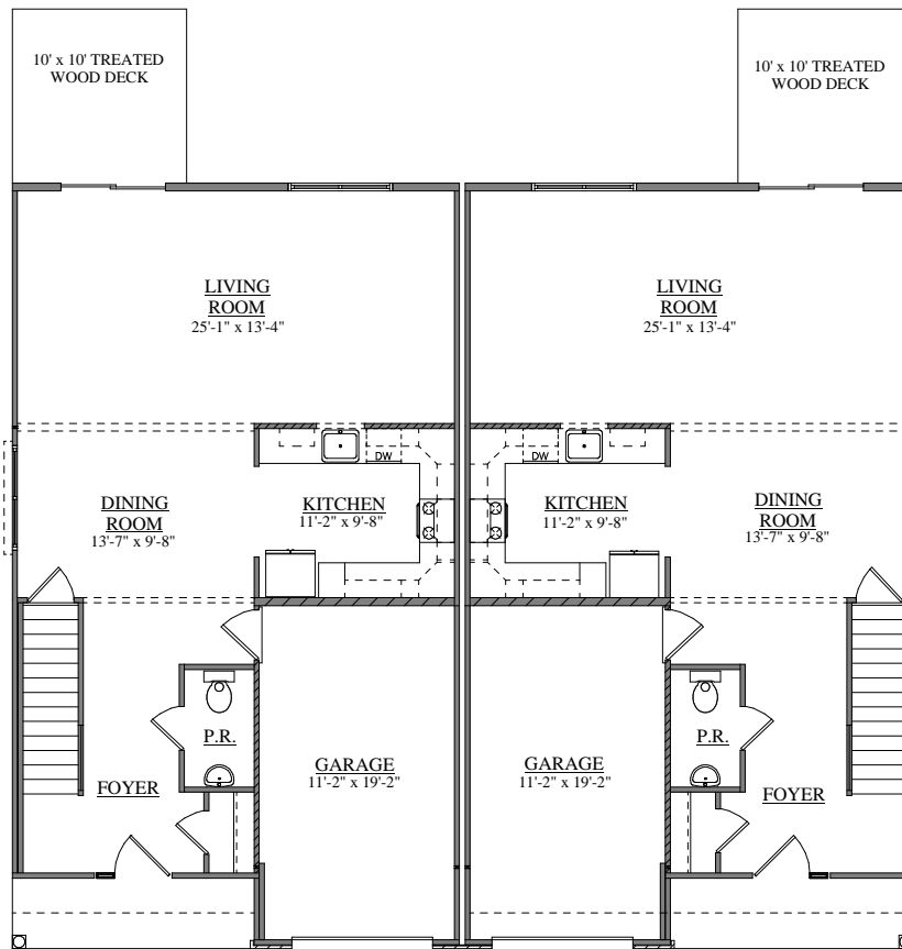
FIRST FLOOR PLAN FORINO - BERKELEY II TOWNHOUSE
