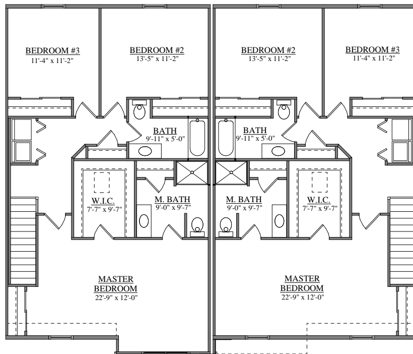
SECOND FLOOR PLAN FORINO - BERKELEY II TOWNHOUSE
