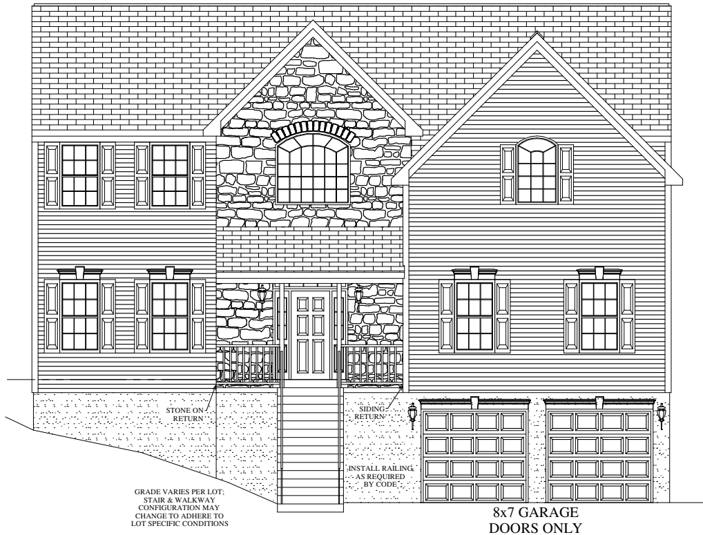
FRONT ELEVATION FORINO - BOSTON BASEMENT ENTRY - STANDARD CLASSIC 3307 SQ. FT.
