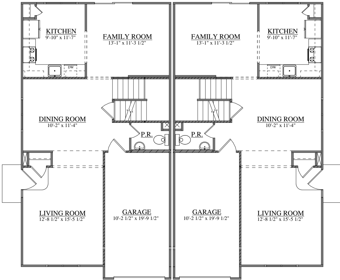
FIRST FLOOR PLAN FORINO - CAROLINA - DUPLEX
