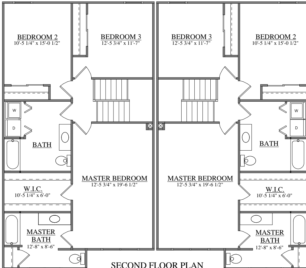
SECOND FLOOR PLAN FORINO - CAROLINA - DUPLEX
