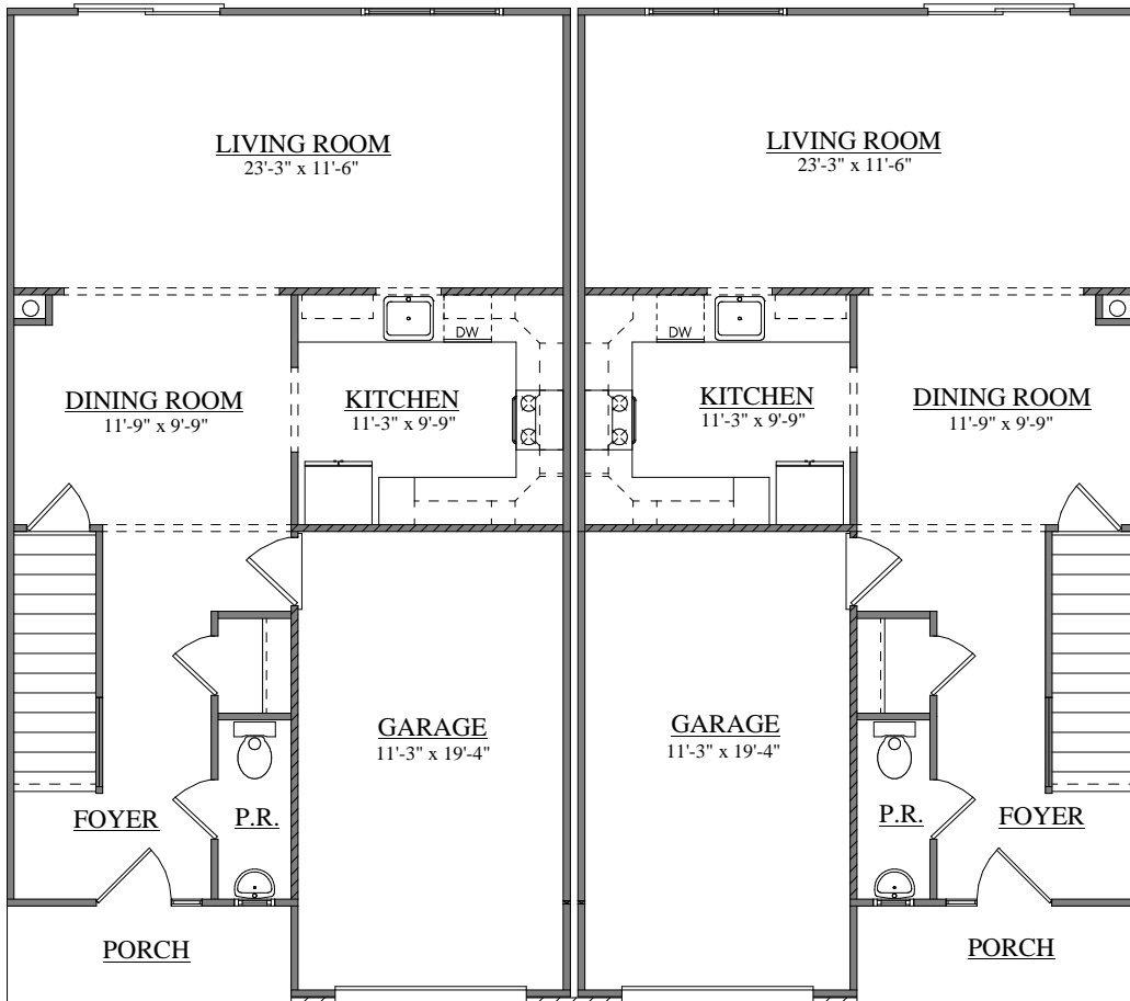
FIRST FLOOR PLAN FORINO - COLUMBIA DUPLEX
