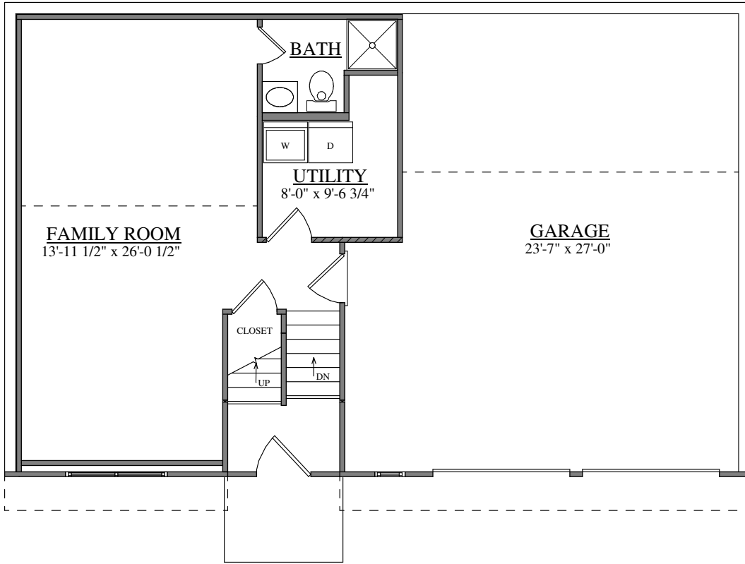
LOWER LEVEL PLAN FORINO - DELAWARE II - POURED
