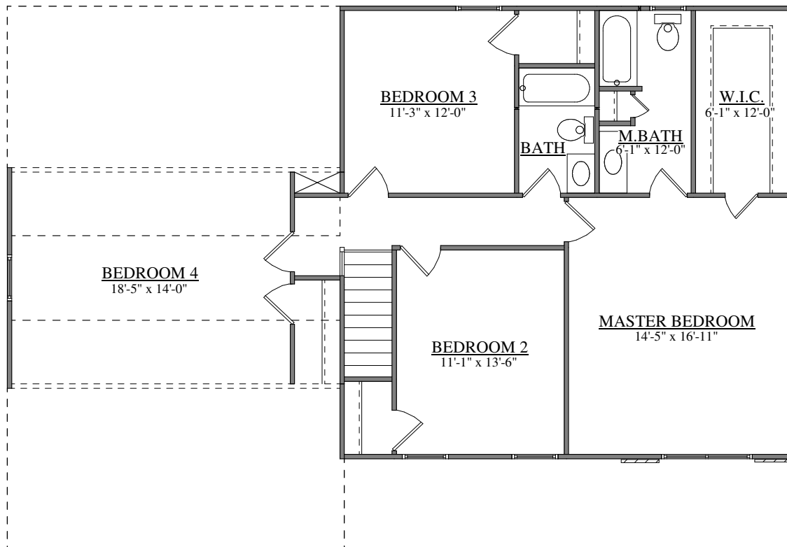
SECOND FLOOR PLAN FORINO - DENVER III - 4BR
