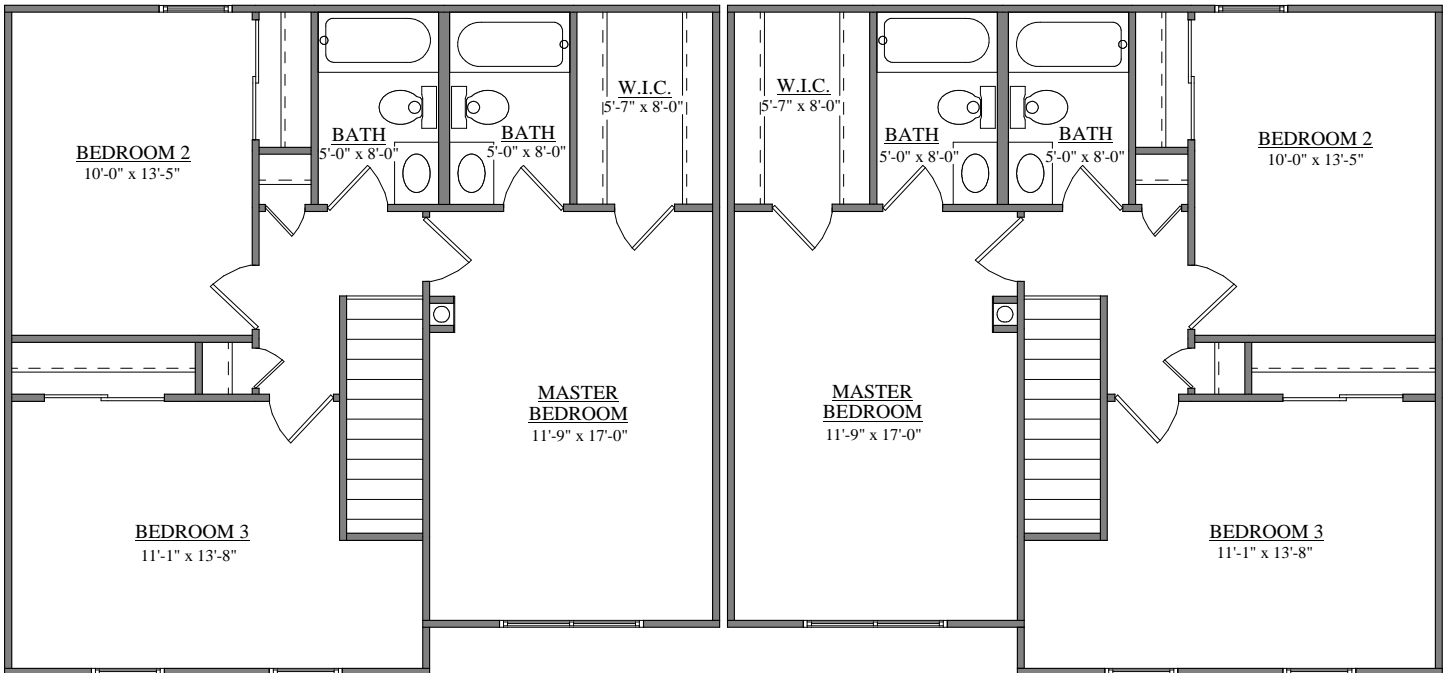
SECOND FLOOR PLAN FORINO - GEORGIAN DUPLEX
