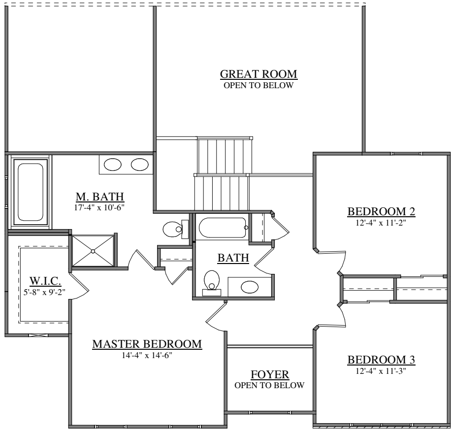
SECOND FLOOR PLAN FORINO - IOWA III
