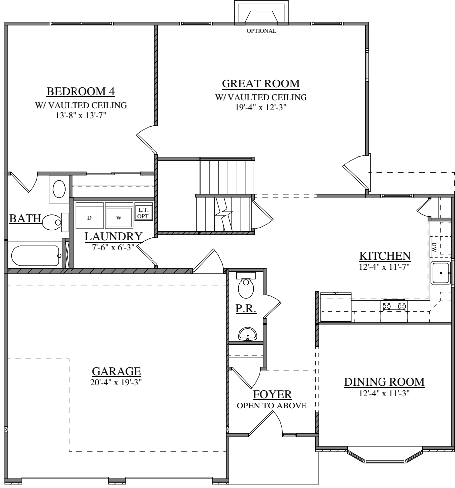
FIRST FLOOR PLAN FORINO - IOWA III
