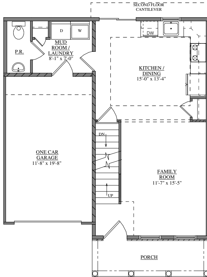
FIRST FLOOR PLAN FORINO - LIBERTY II
