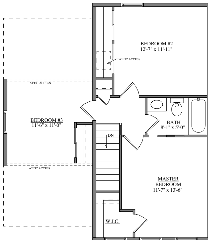
SECOND FLOOR PLAN FORINO - LIBERTY II
