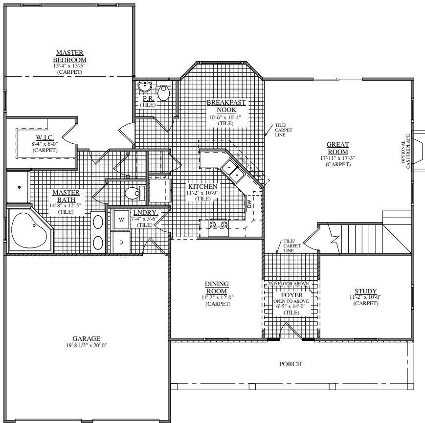
FIRST FLOOR PLAN FORINO - THE MORGAN (SC#2)
