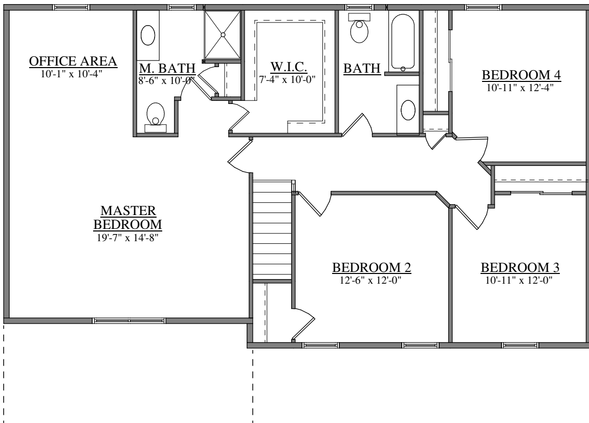
SECOND FLOOR PLAN FORINO - MILLVILLE I
