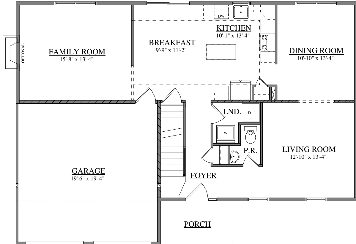
FIRST FLOOR PLAN FORINO - MILLVILLE I
