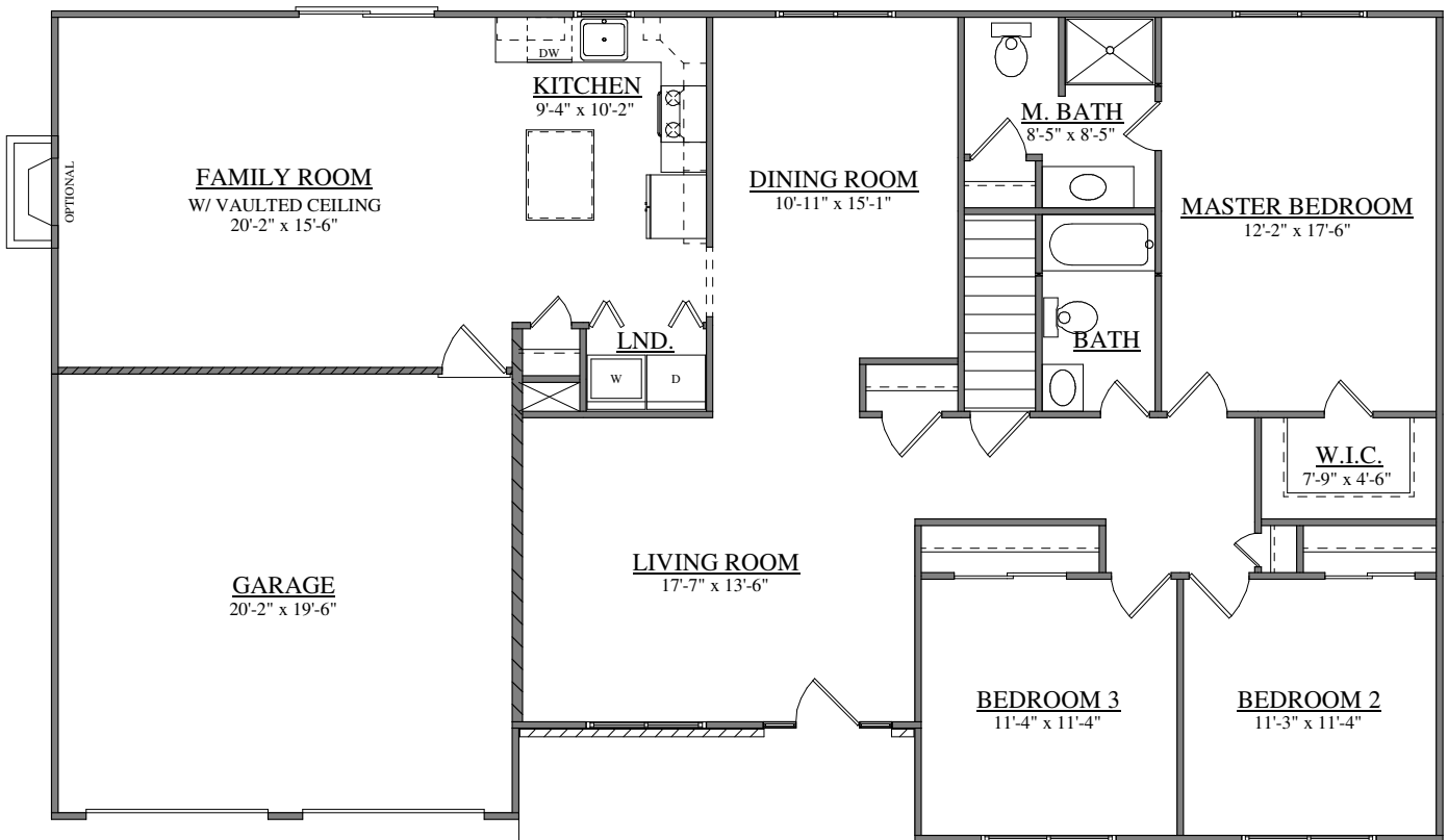
FIRST FLOOR PLAN FORINO - NEVADA
