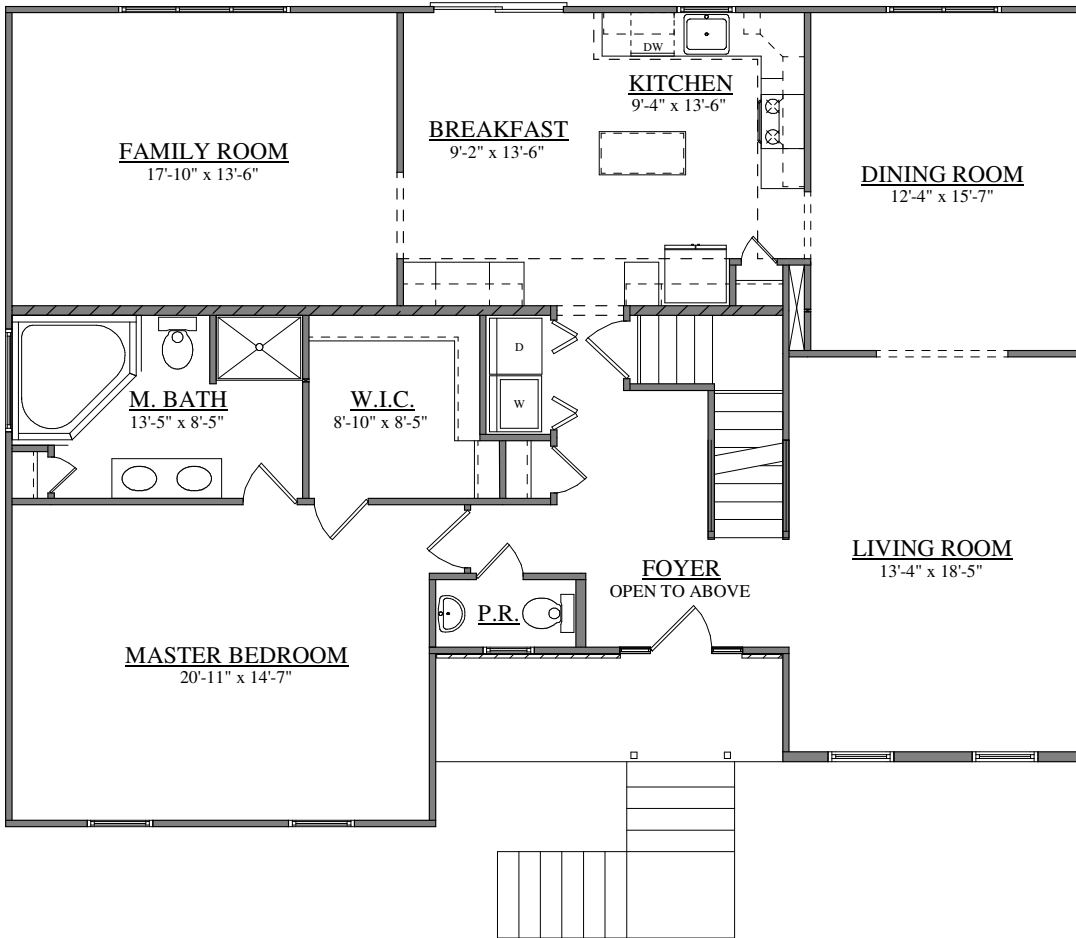
FIRST FLOOR PLAN FORINO - NEW BEDFORD
