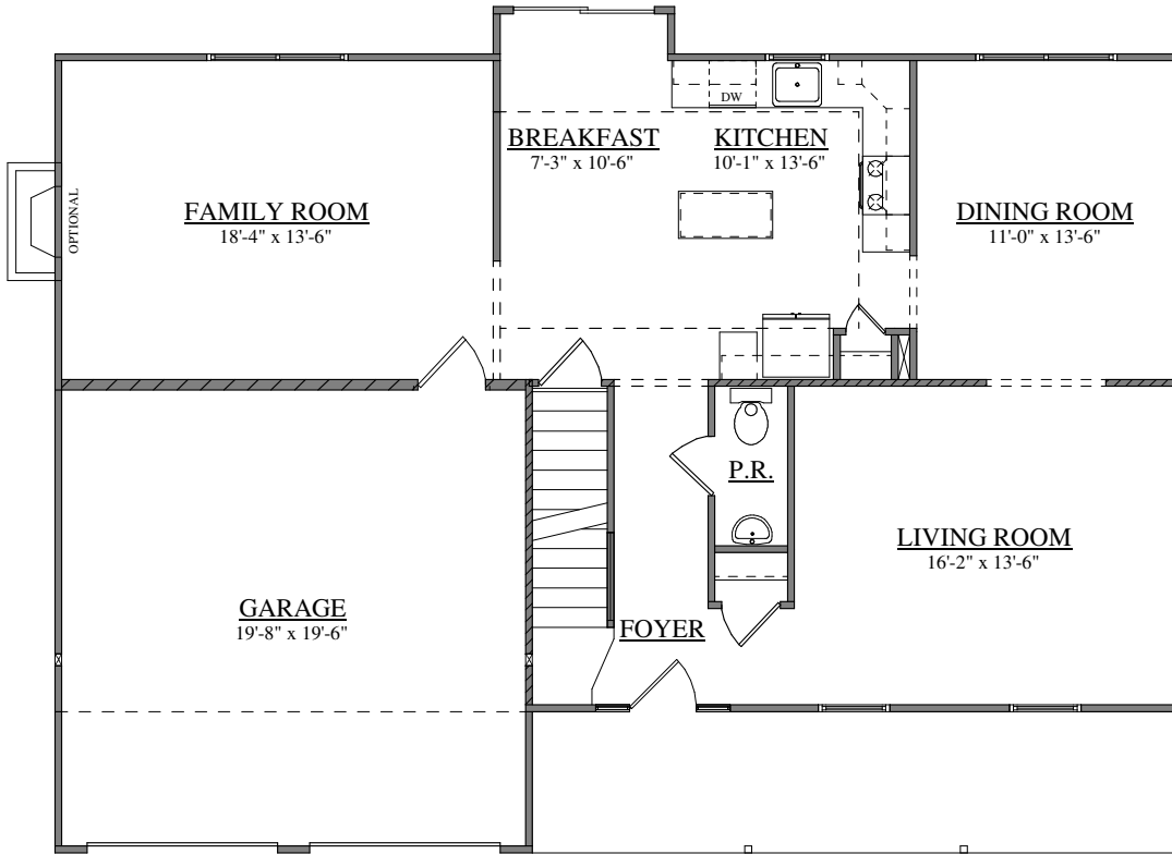
FIRST FLOOR PLAN FORINO - NEW JERSEY I
