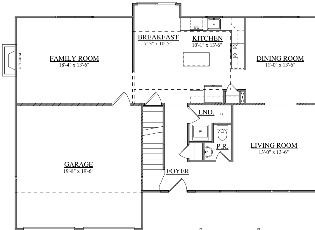
FIRST FLOOR PLAN FORINO - NEW JERSEY II
