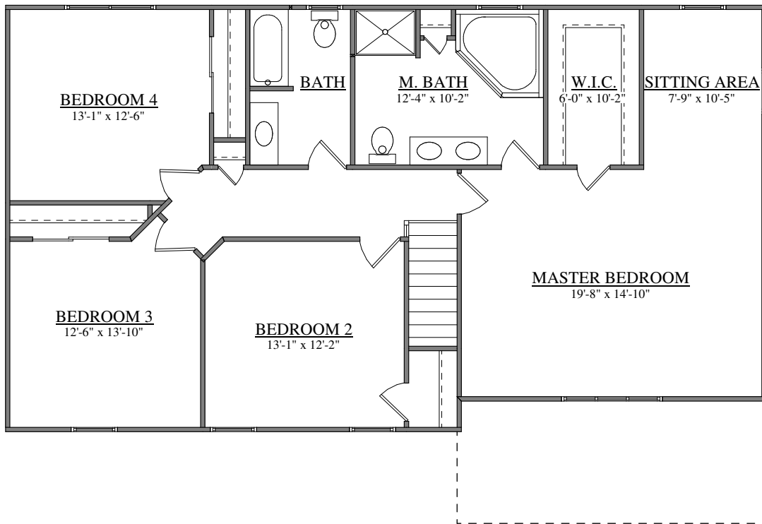
SECOND FLOOR PLAN FORINO - NEW JERSEY III
