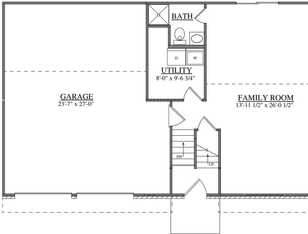
LOWER LEVEL PLAN FORINO - PENNSYLVANIA - SLAB
