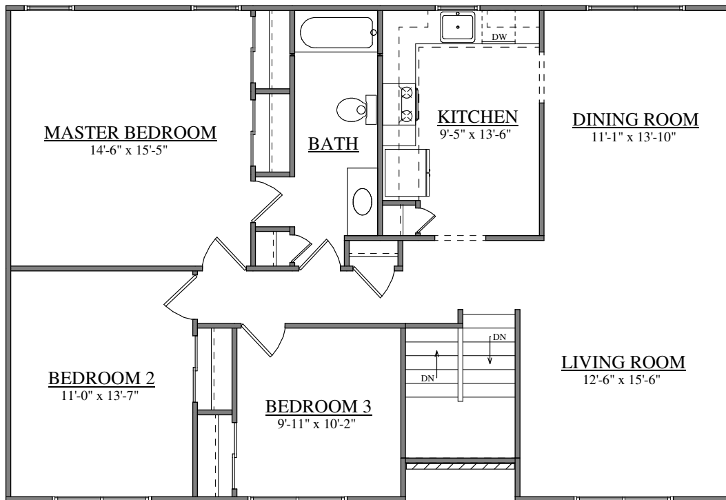
UPPER LEVEL PLAN FORINO - PENNSYLVANIA - SLAB
