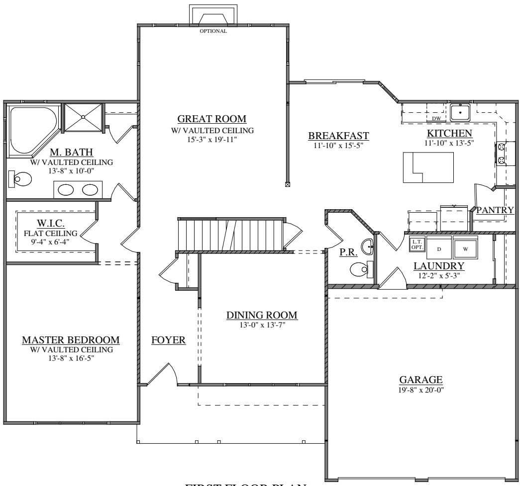
FIRST FLOOR PLAN FORINO - RHODE ISLAND
