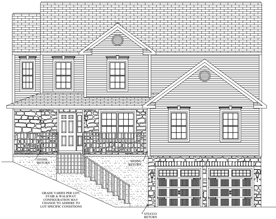
FRONT ELEVATION FORINO - SAN DIEGO - BASEMENT ENTRY - OPTION "A" 2646 SQ.FT.
