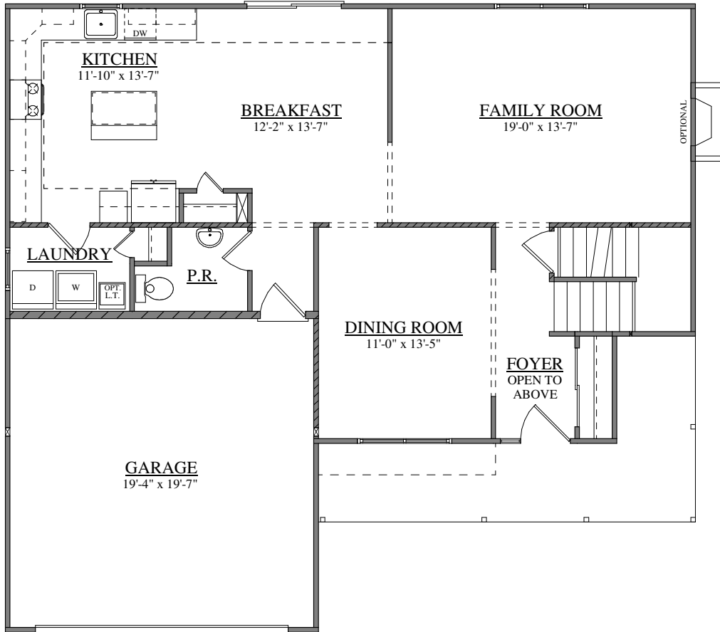
FIRST FLOOR PLAN FORINO - SAN DIEGO
