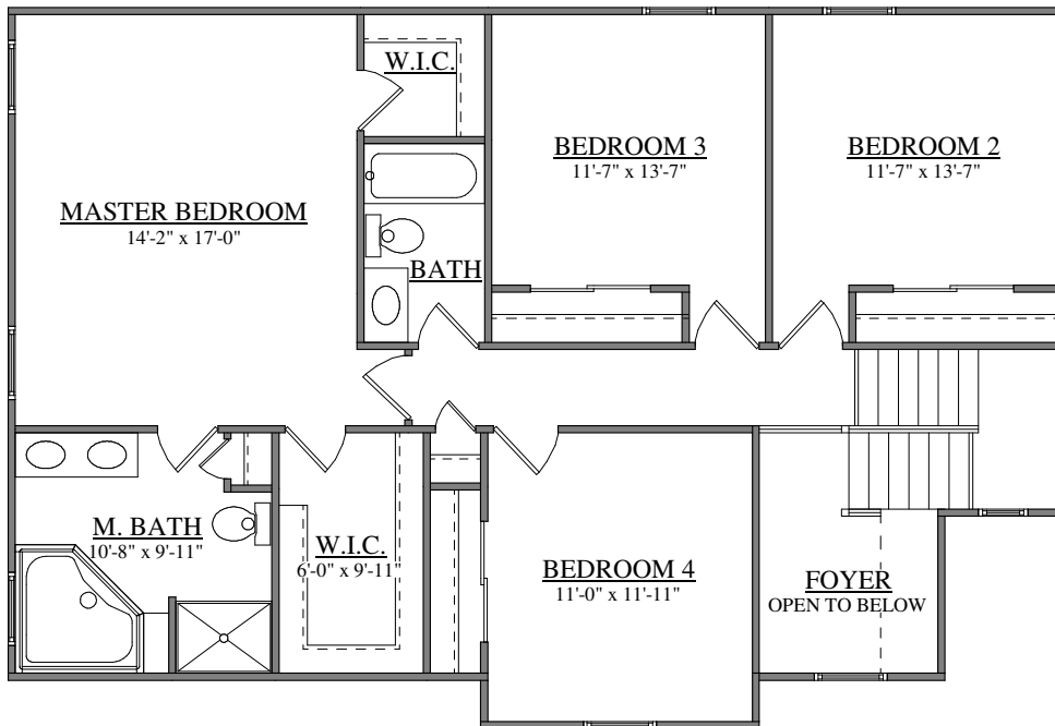
SECOND FLOOR PLAN FORINO - SAN DIEGO
