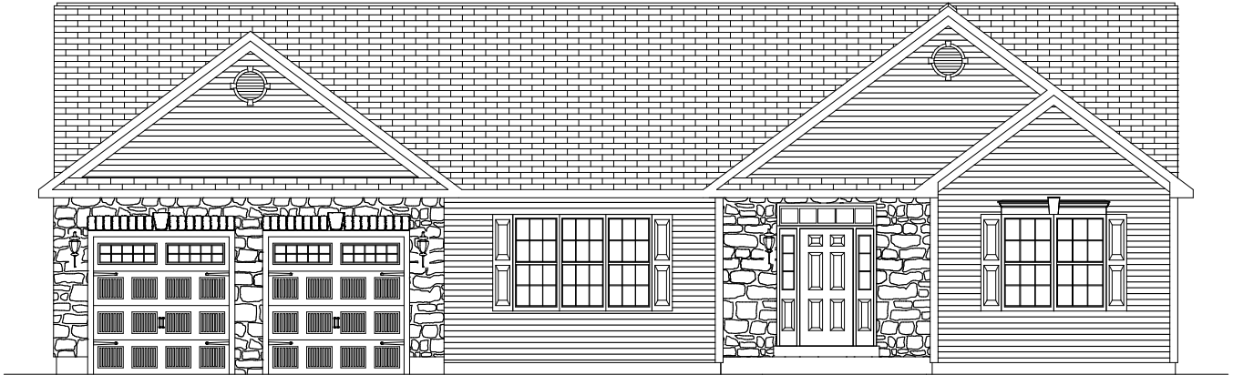
FRONT ELEVATION FORINO - SARASOTA - STANDARD CLASSIC 2330 SQ.FT.
