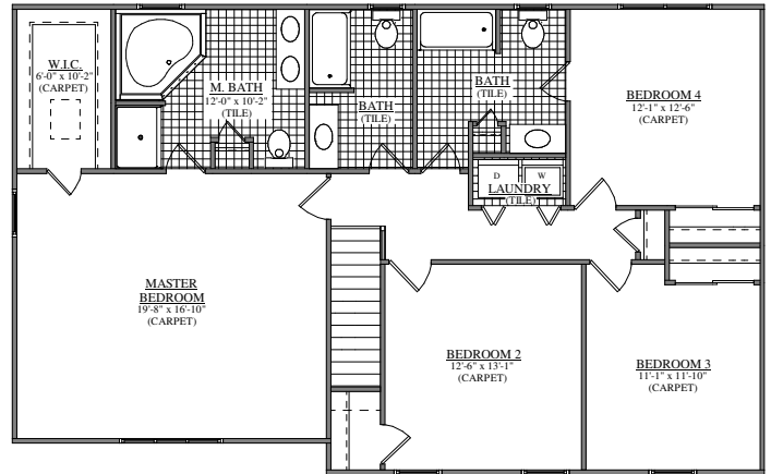
SECOND FLOOR PLAN FORINO - THE SENECA (S.C. #6) W/ OPTIONAL 3RD BATH
