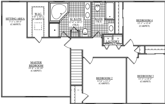
SECOND FLOOR PLAN FORINO - THE SENECA (S.C. #6)
