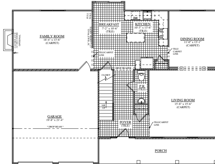
FIRST FLOOR PLAN FORINO - THE SENECA (S.C. #6)
