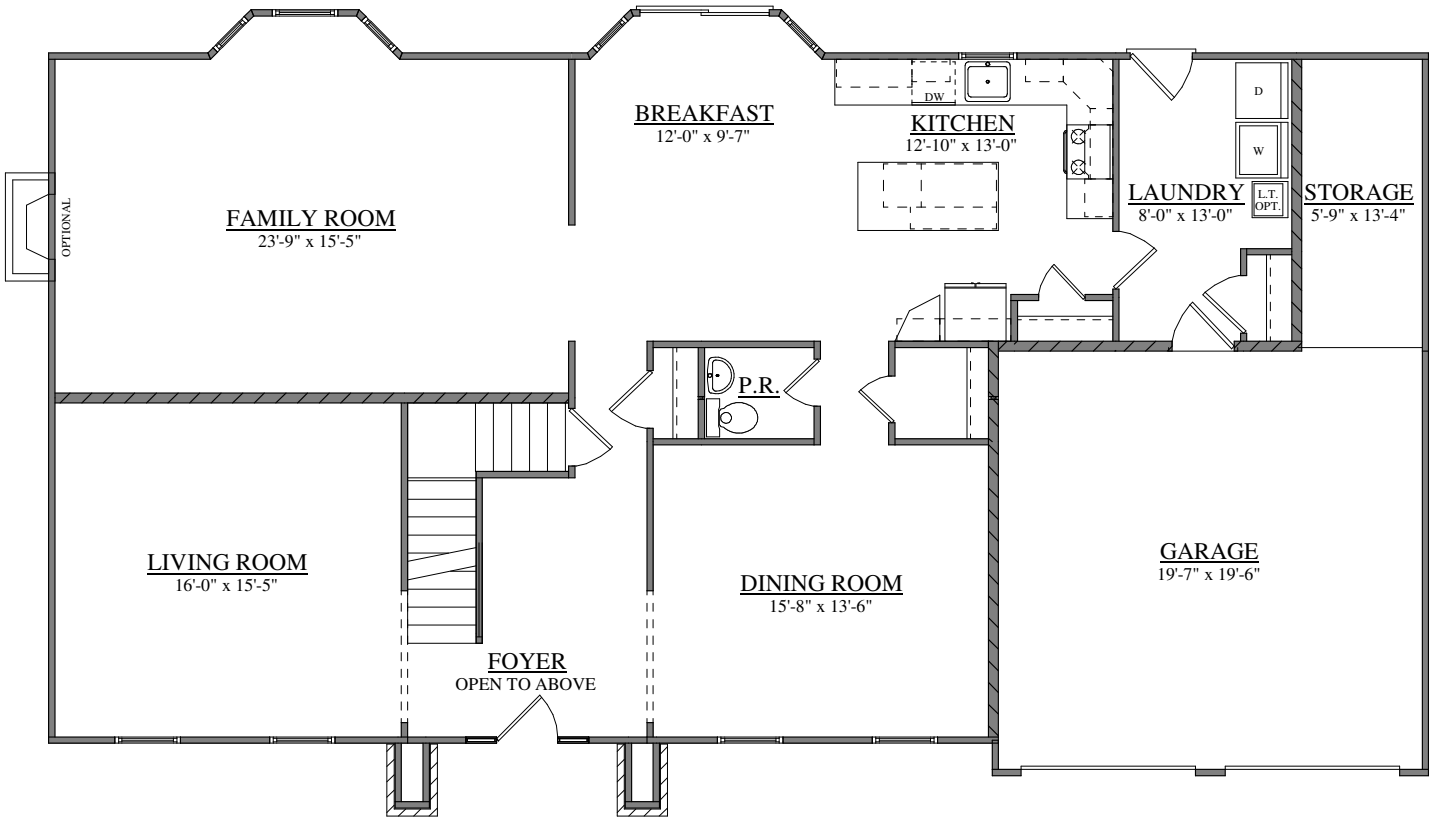
FIRST FLOOR PLAN FORINO - ST. CLAIR
