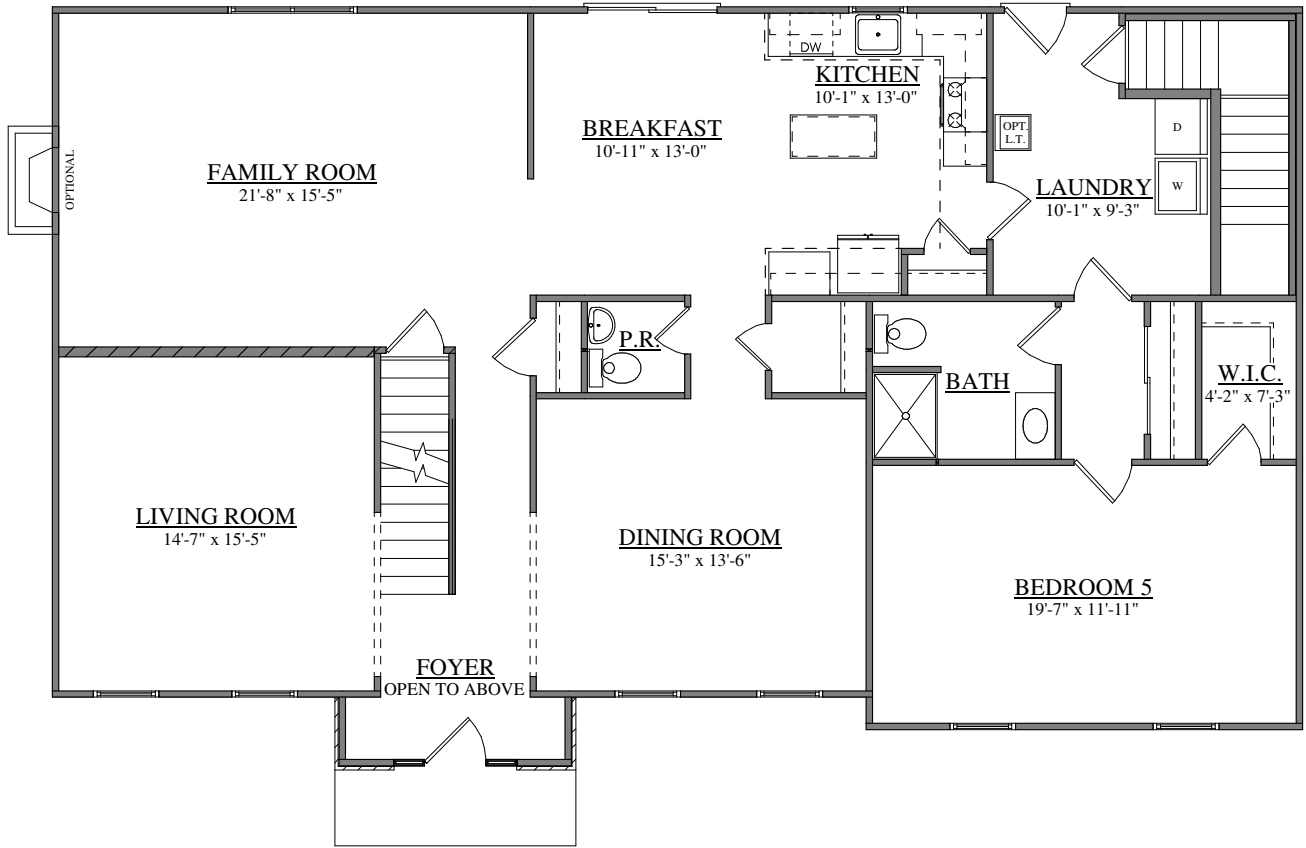
FIRST FLOOR PLAN FORINO - ST. PAUL B.E.
