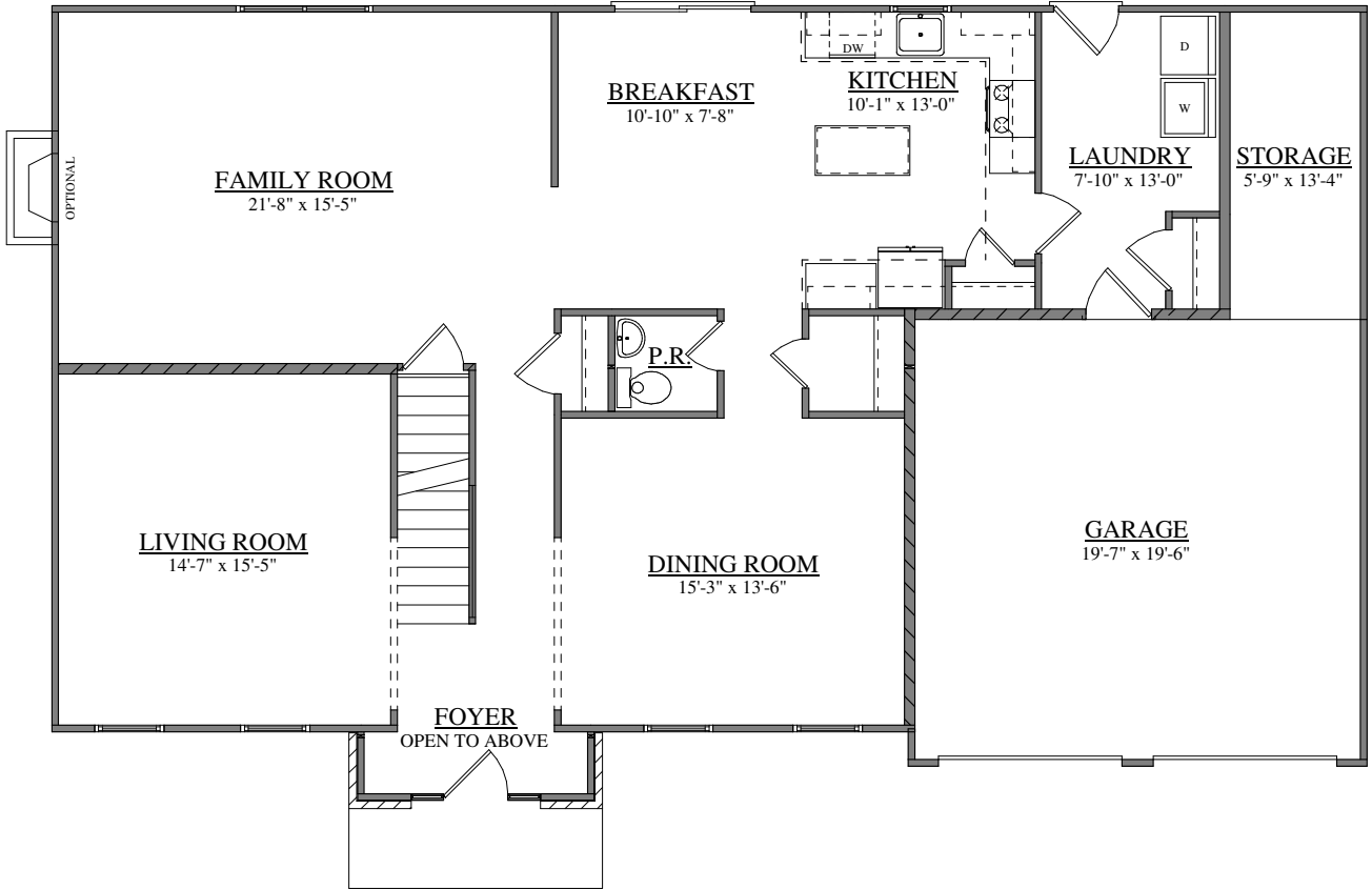
FIRST FLOOR PLAN FORINO - ST. PAUL
