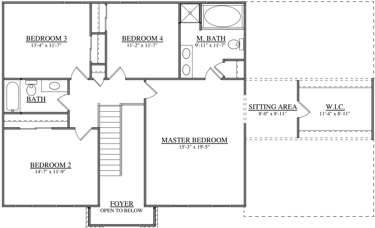
SECOND FLOOR PLAN FORINO - ST. PAUL
