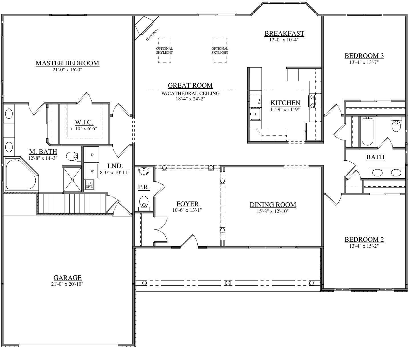
FIRST FLOOR PLAN FORINO - TAHOE III
