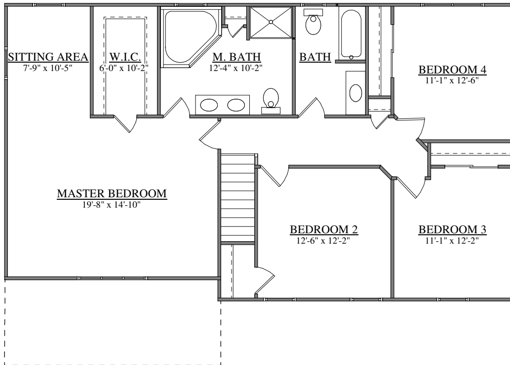
SECOND FLOOR PLAN FORINO - TRENTON
