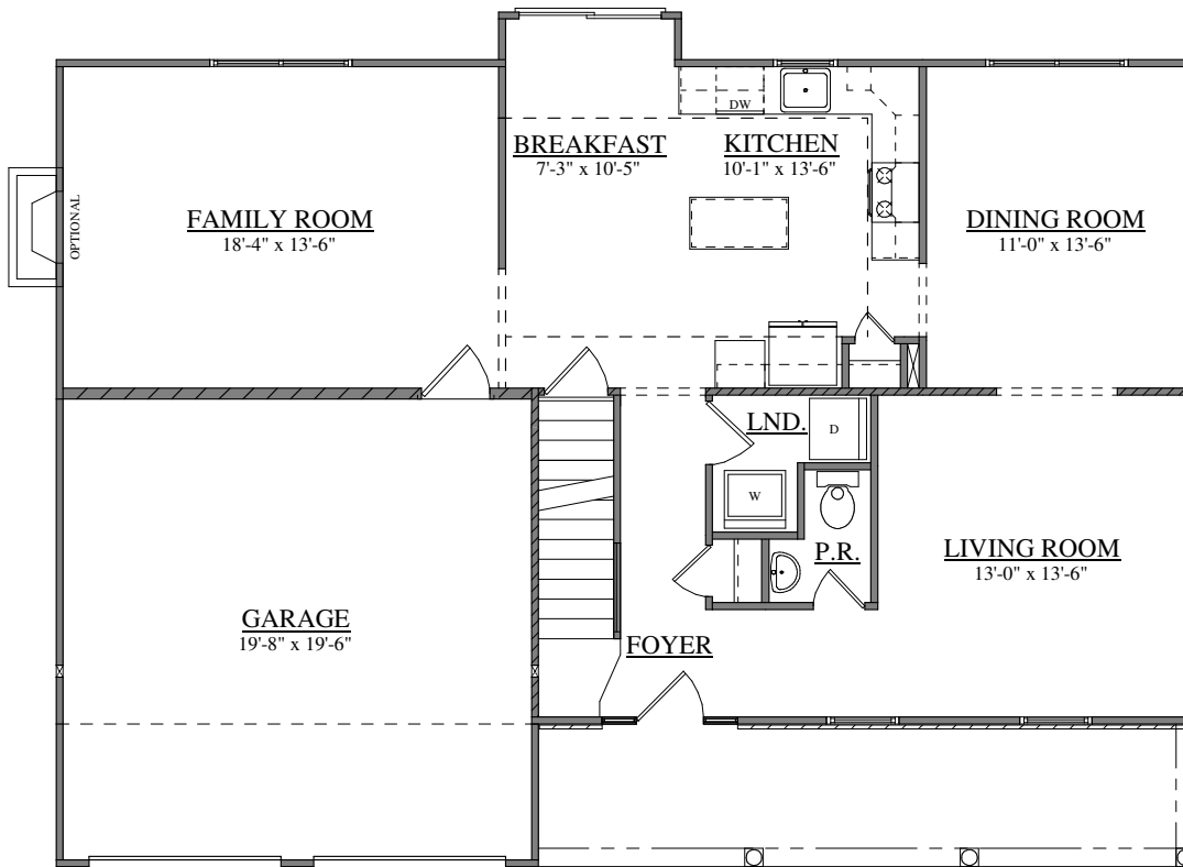
FIRST FLOOR PLAN FORINO - TRENTON
