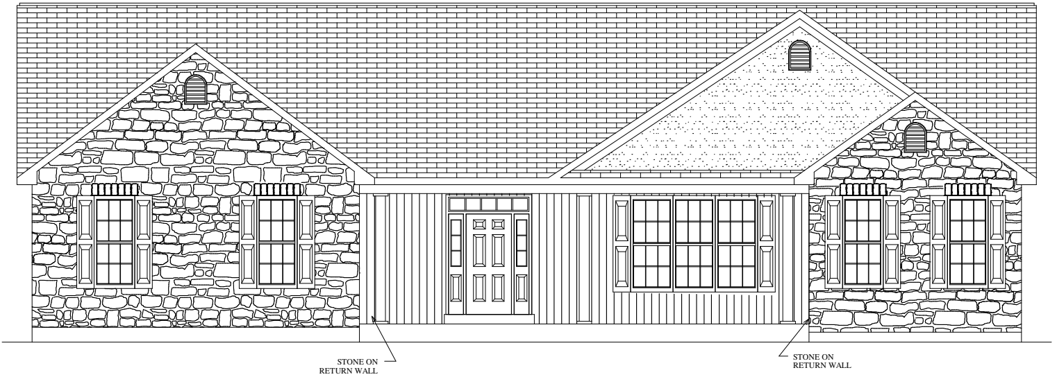
FRONT ELEVATION FORINO - TAHOE III - CRICKET SLOPE FARMS 2479 SQ. FT.
