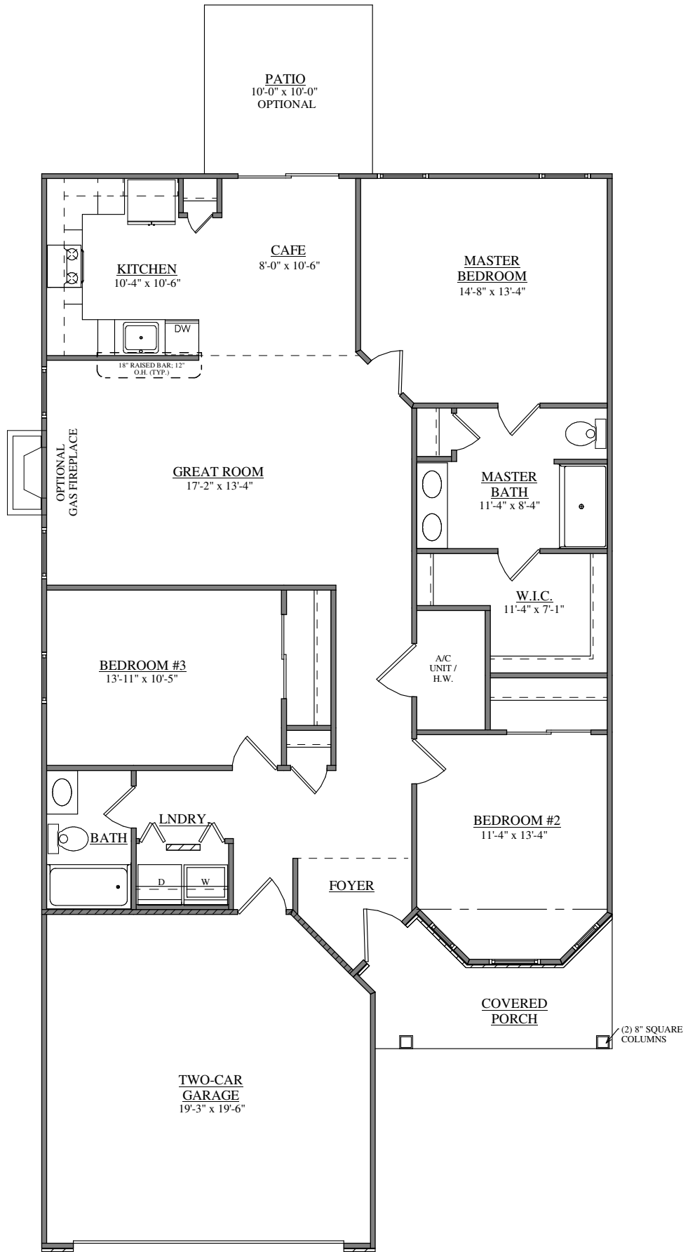
FIRST FLOOR PLAN FORINO - WILLIAMSBURG I (SLAB) - CLASSIC
