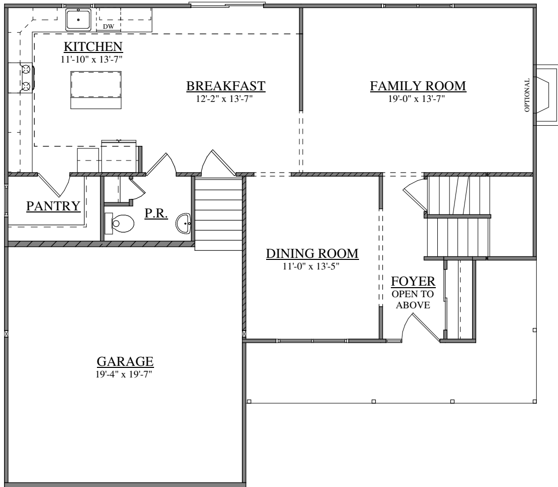
FIRST FLOOR PLAN FORINO - SAN DIEGO II
