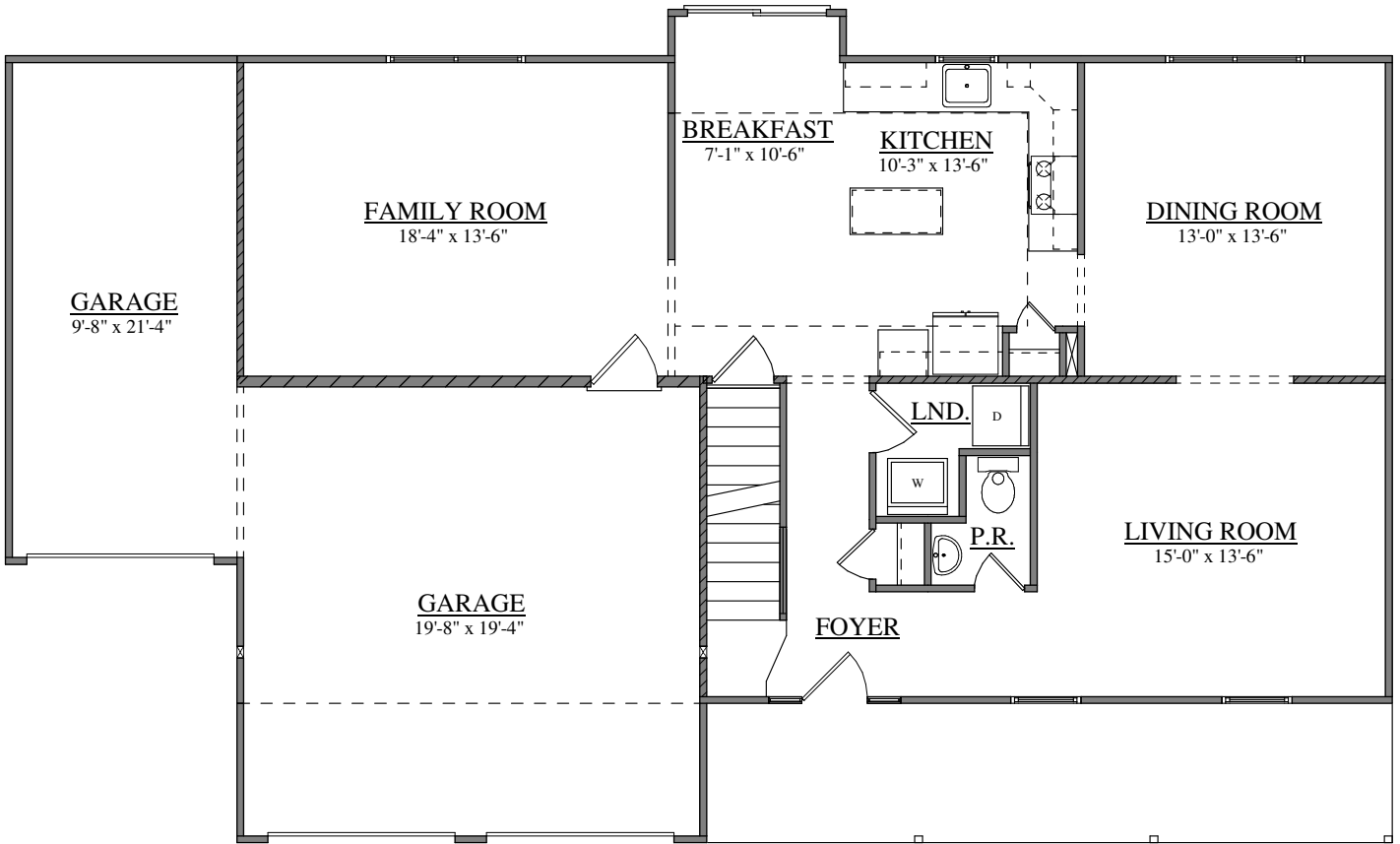
FIRST FLOOR PLAN FORINO - SOMERSET
