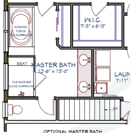
OPTIONAL MASTER BATH W/ TILE SHOWER W/ GLASS SURROUND
