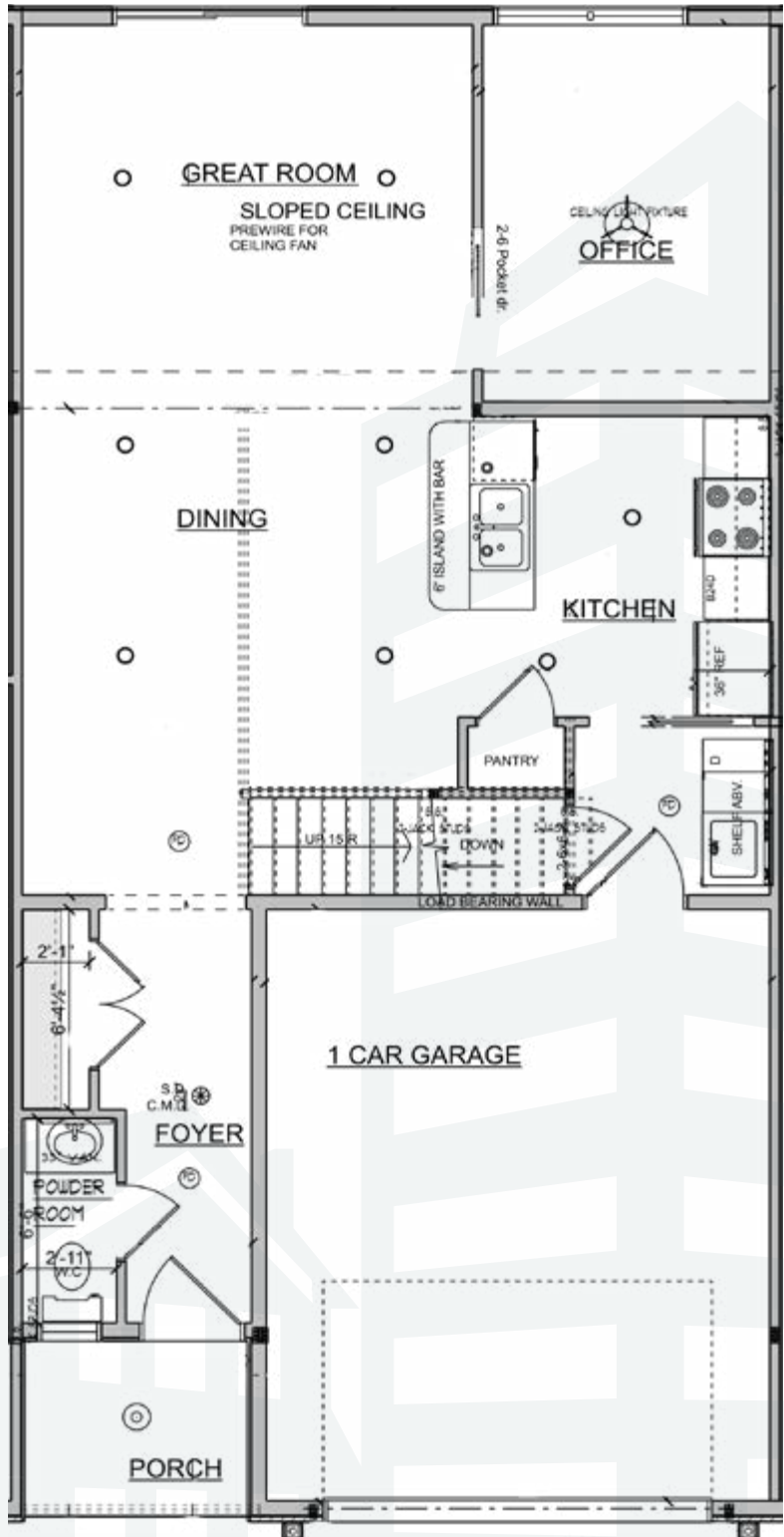
First Floor
