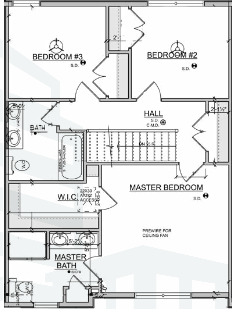
Second Floor
